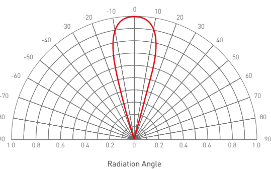
Radiation Characteristics
